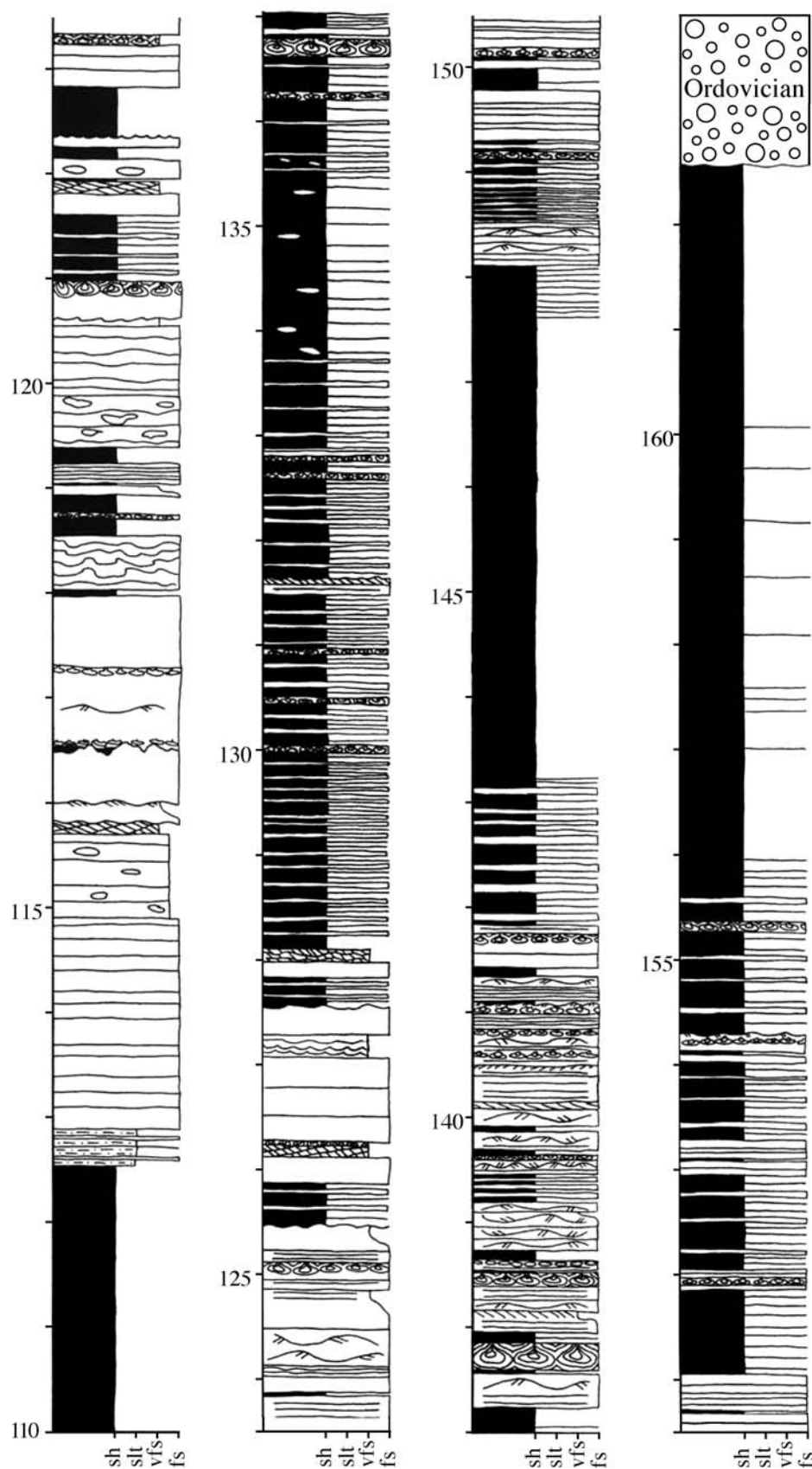
FIG. 12.—Stratigraphic column of the Kurgikh Formation at the KU2 section. Section covers the upper 2.5 m of the Surichun Member and the entire Kuru Member. Lithologic scale: sh = shale, slt = siltstone, vfs = very fine sandstone, fs = fine sandstone. See Figure 4 for legend for symbols.
