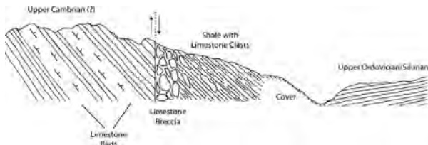
Figure 5. Sketch of the inferred geology of the upper part of the Wachi La section (above about 340 m; see Fig. 3) showing the top of the measured section, a fault with associated fault breccia, and overlying apparently Ordovician carbonate strata with different strike and dip. The fault itself is poorly exposed. The sketch is approximately orientated east–west, with east on the right.
