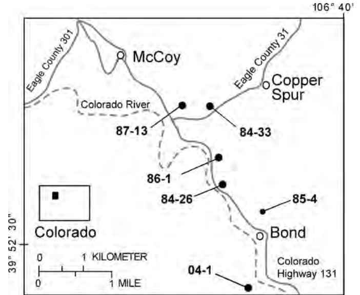
FIG. 2.—Locality map of study area. Outcrop locality numbers used in this study are from Houck (1993).
