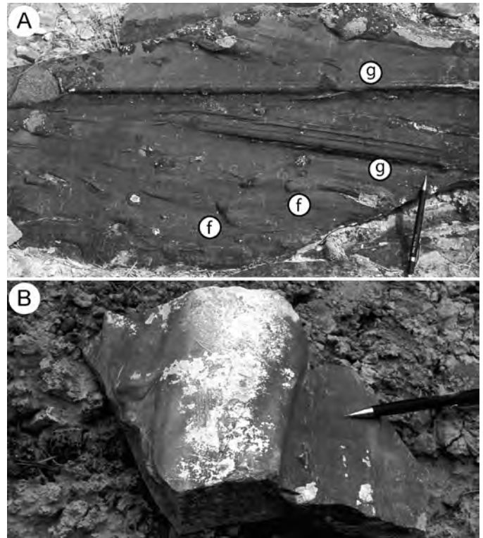
FIG. 9.— A ) Large grooves (g) and flute marks (f) on base of HCS sandstone at 31.81 m of section 84-33 (Fig. 4). B ) Large gutter cast from base of same bed as shown in Part A. Pencil is 14 cm long.
