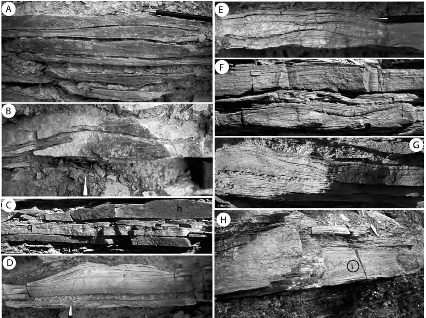
FIG. 5.— A ) Small-scale HCS from 6.3 to 6.8 m in Section 86-1. B ) Combined-flow-ripple lamination from 3.29 m of section 84-33. Note nearly symmetrical cross section, rounded crest, and convex-up foresets. C ) Quasi-planar laminated (q) and HCS (h) beds from 3.1 m of section 84-26. D ) Parallel lamination and well-preserved hummocky bedform from Section 84-33. E ) Combined-flow-ripple lamination from 5.61 m of section 84-33. F ) Lower bed with combined-flow-ripple lamination and draping lamination and upper bed with parallel lamination from 14.85 m of Section 84-26. G ) Three-dimensional view of small asymmetric hummocky bedform from 2.01 m at Section 87-13. Ripple-scale bedform at top of hummock in upper left shows migration to south, reflecting migration under combined flow. H ) Thick, large-scale HCS bed from an unmapped outcropping 3.5 km east of McCoy, CO. Pencil for scale is circled. Pencil in photos is 14 cm long and tip is 2 m long.
