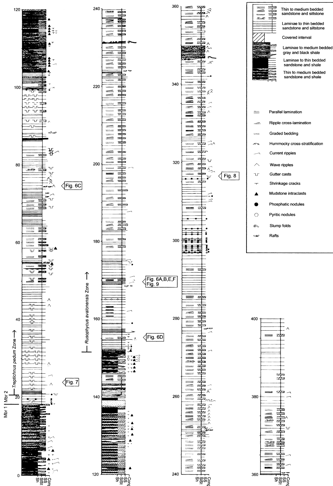
FIGURE 3 —Stratigraphic section for member 2 at Fortune, showing major sedimentological features and range of Treptichnus pedum and Rusophycus avalonensis Zones. Boxes enclosing figure numbers refer to stratigraphic position of material figured in this paper. Section based on Myrow and Hiscott (1991, fig. 3). Note: Figures 6A, B, E, F and Fig. 9 are from the Grand Bank Locality and are tied in to the Fortune Section at approximately 170 meters based on sedimentological and stratigraphic evidence.
