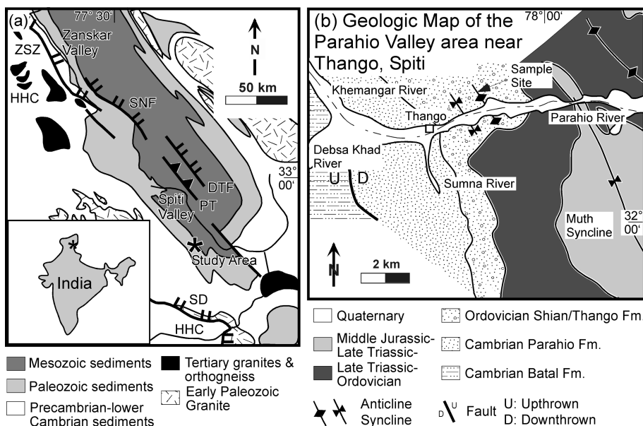
Fig. 2. (a) Geology of the Spiti–Zanskar basin area showing the location of sampling site in Spiti (after Wyss et al. 1999). Inset shows the location of the map on a regional scale in India (modified from Draganits et al. 2004; Paulsen et al. 2007). (b) Geologic map showing sample site in Parahio Valley in Spiti (compiled and modified from Fuchs 1982; Bhargava & Bassi 1998; Wiesmayr & Grasemann 2002; Myrow et al. 2006b; Paulsen et al. 2007). DTF, Dutung–Thaktote Fault; HHC, High Himalayan Crystallines; PT, Parang La Thrust; SNF, Sarchu Normal Fault; SD, Sangla Detachment; ZSZ, Zanskar Shear Zone.
