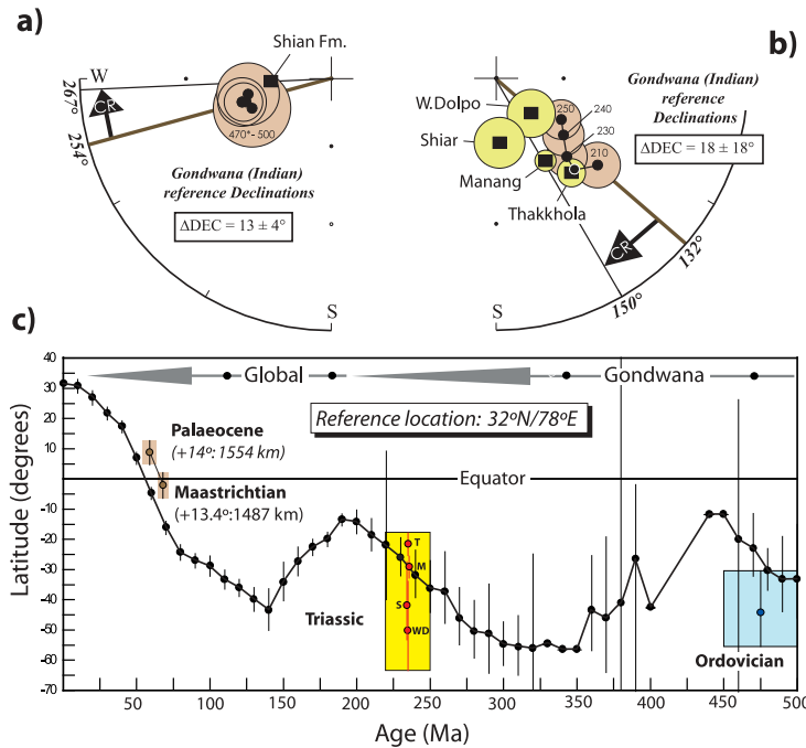
Fig. 6. (a) Ordovician mean directions from Gondwana rotated to an Indian reference frame (calculated from Torsvik & Van der Voo 2002; Torsvik et al. 2008, table 3) and compared with the Shian Formation direction (black square). Gondwana mean directions are calculated without the 463 Ma Salala Ring Complex (470–500 Ma; Table 2). (b) Primary Triassic directions (with yellow \alpha_{95} ovals) from the Western Dolpo (WD), Thakkhola (T), Manang (M) and Shiar (S, Crouzet et al. 2003, table 4) compared with Gondwana reference data. The average reference declination is a mean of 250–210 Ma directions. In stereo-plots closed symbols denote positive inclinations. Reference directions are shown with brown A95 circles. All data are recalculated to a common location in Spiti (32°N, 78°E). CR, clockwise rotation compared with Gondwana reference frame. (c) Stable India reference latitude curve (recalculated to Spiti location) based on Gondwana (500–220 Ma; Torsvik & Van der Voo 2002) and global (190–0 Ma; Torsvik et al. 2008) palaeomagnetic reference frames. It should be noted that Ordovician and Triassic data from the Tethyan Himalaya on average yield lower latitudes than stable India but they statistically overlap. Conversely, Maastrichtian (c. 68 Ma) and Palaeocene (c. 59 Ma) data from the Tethyan Himalaya (Gamba and Duela regions) plot systematically to the north of the reference curve and imply 1500 km of younger shortening between the Tethyan Himalaya and cratonic India (see also Patzelt et al. 1996).
